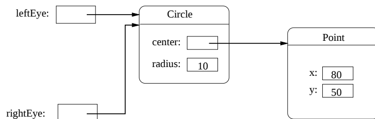
Figure 5.6: Variables leftEye and rightEye are aliases.
